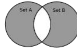
Symmetric Difference
