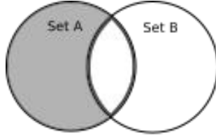
Difference
