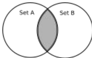
Intersection
